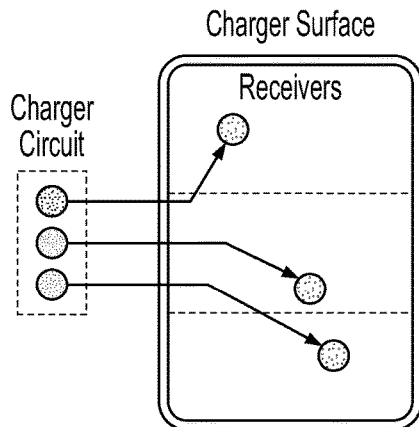
c-Single Protocol Geo-Cast: One Charger Sub-unit per Pre-Designated Section of Charger Surface - Only Supports One Protocol, Voltage, and / or Power Level
