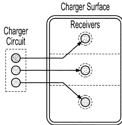
b-Multi-Protocol - Tightly Coupled: One Charger Sub-unit per Single Receiver in Fixed Position; Can be Different Protocols, Voltages, and / or Power Levels
