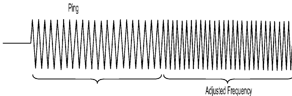
Voltage Applied to Charger Coil
